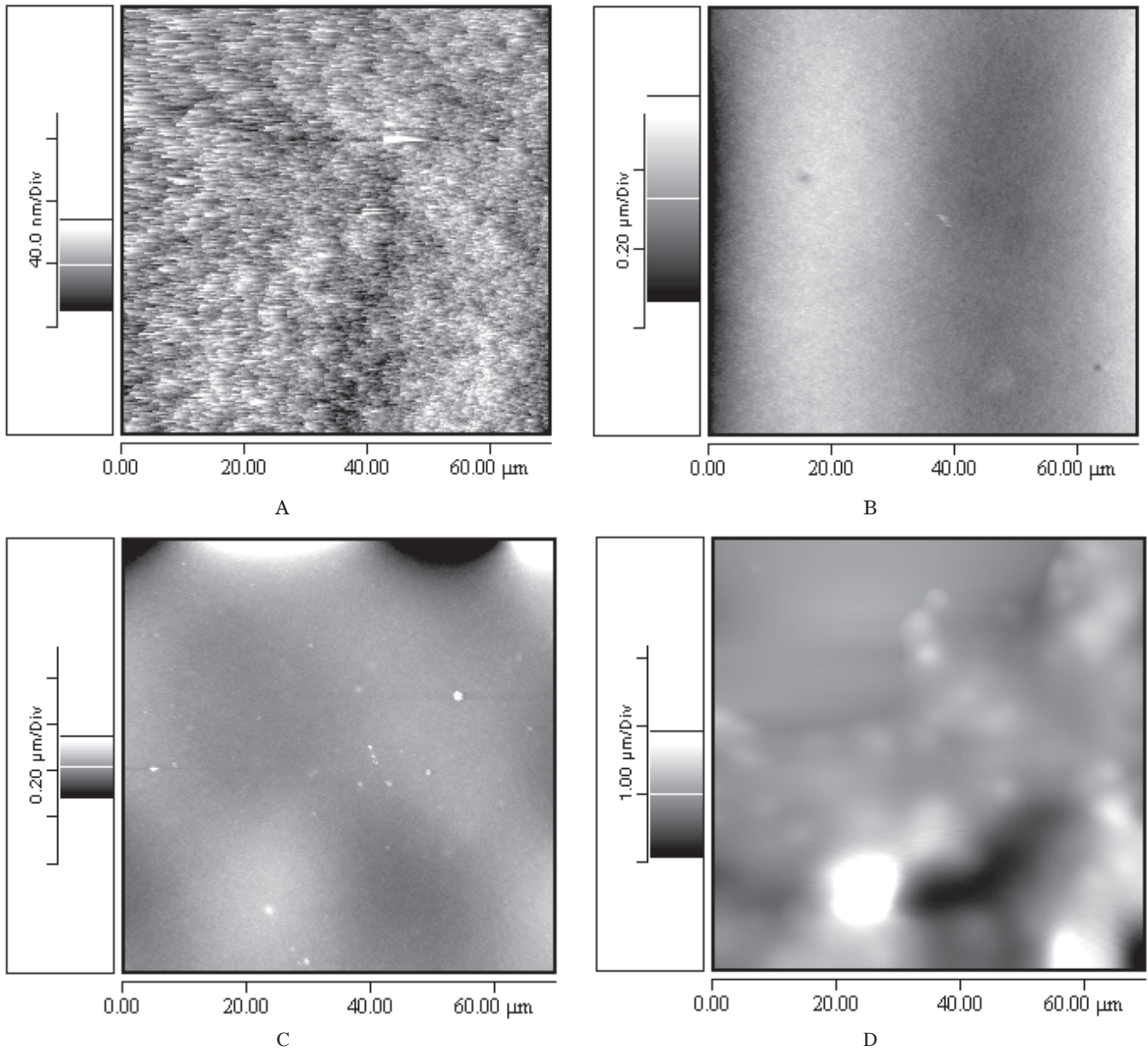
Figure 1. AFM images of paper topography: Epson Glossy (A-upper left), Epson Luster (B-upper right), Kodak Gloss (C-lower left), and Kodak Satin (D-lower right).
