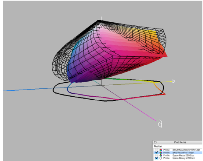
Figure 2. EPSON Stylus P2200 Gloss paper and FUJI PictroProof II gamut comparison
