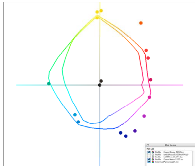
Figure 6. EPSON Stylus P2200 gamut for Matte and Gloss coated vs. test-chart colors.
