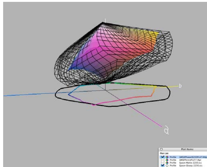
Figure 3. EPSON Stylus P2200 Gloss paper and XEROX Phaser 8200 gamut comparison.
