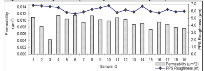
Figure 4: Comparison for Permeability and PPS Roughness
