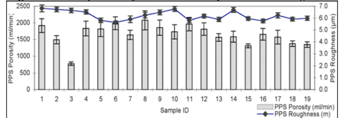
Figure 5: Comparison for PPS Porosity and PPS Roughness.
