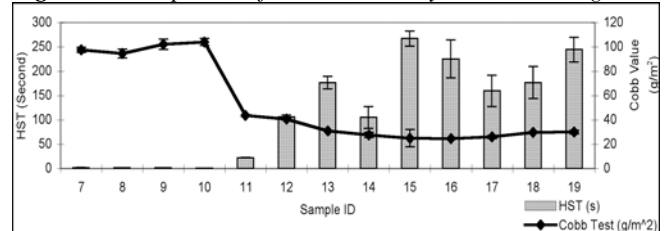
Figure 6: Comparison for Absorption
