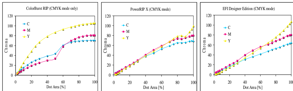
Figure 2: The chroma of CMY vs. Dot area for tested RIP's in CMYK mode (Color Burst RIP – left, PowerRIP X – center, EFI Designer Edition – right)
