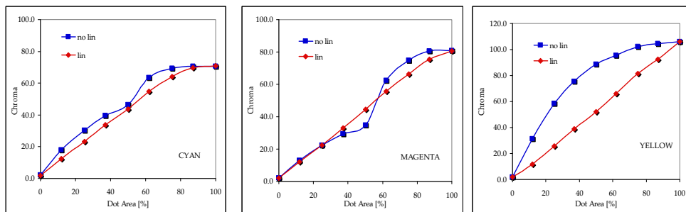
Figure 5: Chroma vs. Dot area for CMYK test charts printed with and without linearization using Monaco Profiler.
