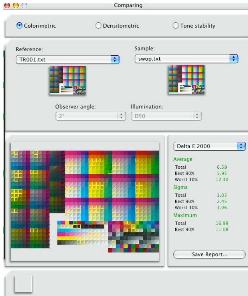
Figure 6. Graphical depiction showing patches of IT8.7/3 chart printed in SWOP mode on the DocuColor 12 that have large \Delta E values relative to TR001.
