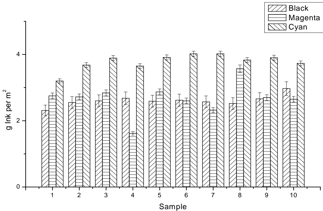
Figure 1: Ink transfer on both sides of different LWC papers.
