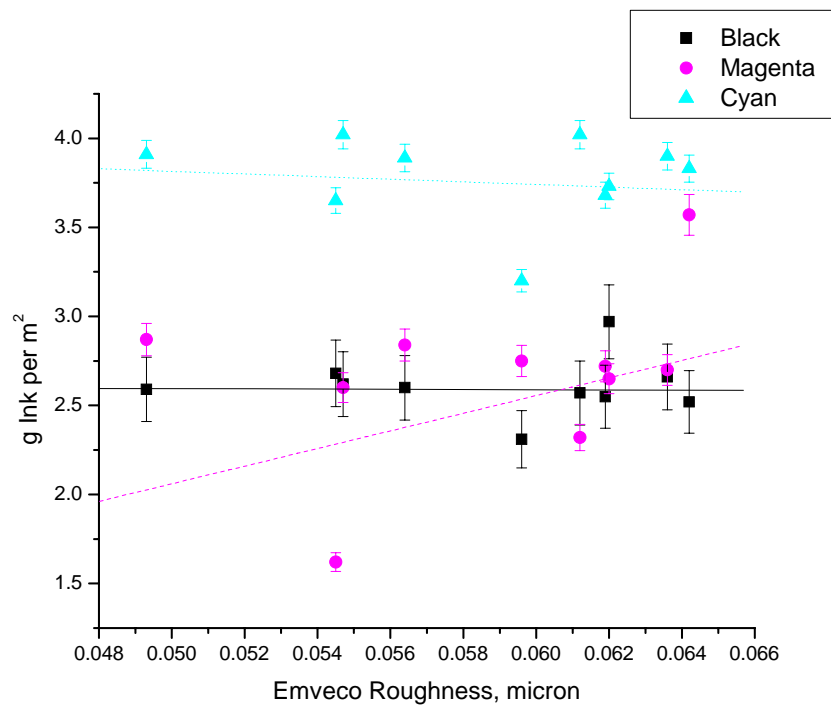
Figure 4: Relationship of ink transfer vs. Emveco roughness.
