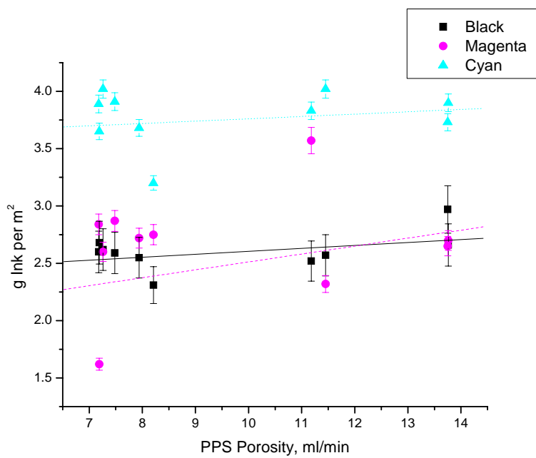
Figure 6: Relationship of ink transfer vs. PPS porosity
