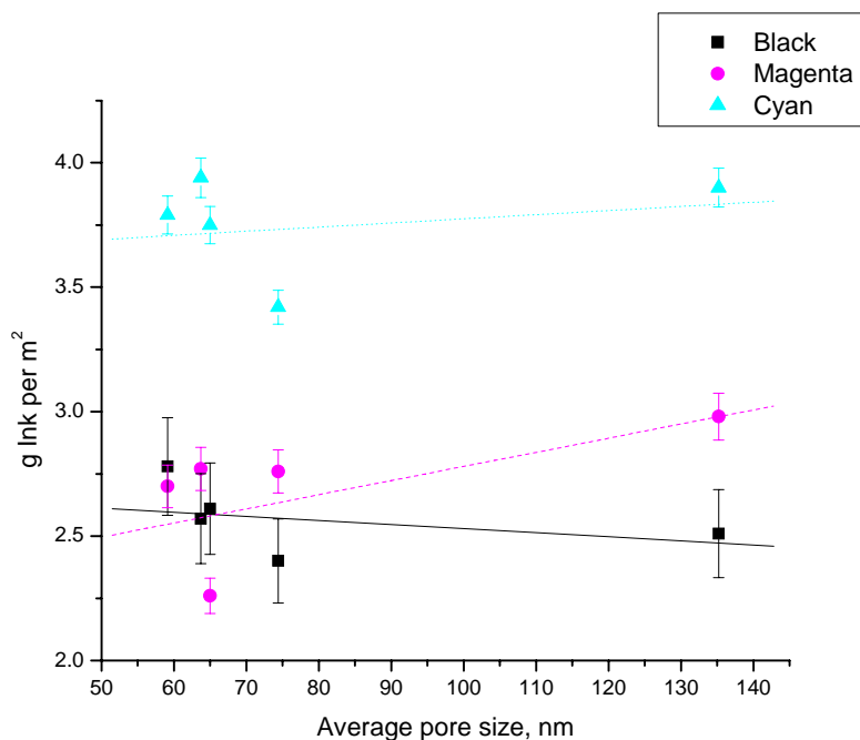
Figure 9: Ink transfer vs. average pore size.
