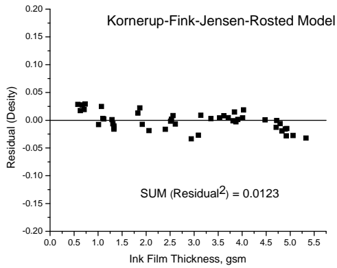
Figure 2. Sum of the square of reflection density residuals and their distribution for various models
