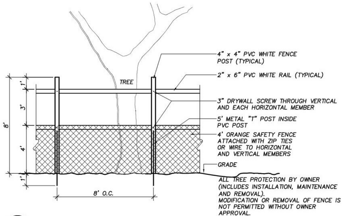
X X-X PVC TREE PROTECTION FENCE— BY OWNER 11/3/08 SCALE: 1/4"=1'-0" M: /LIBRARY/DETAILS/FENCES/TREEPRCT.DWG
