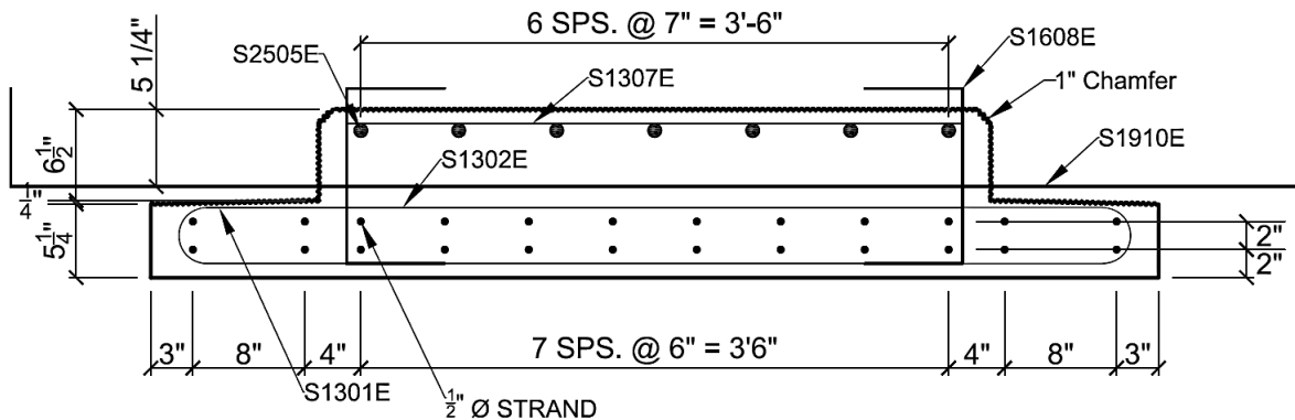
(b) Midspan section
