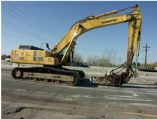
Figure 5-62. Demolition by hammer and pulverizer
