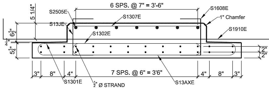
(a) End section
