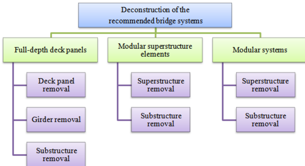
Figure 5-64. Deconstruction hierarchy of the recommended bridge systems
