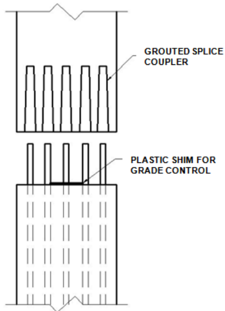
Figure 5-55. Column splice with grouted splice coupler (Source: Culmo 2009)
