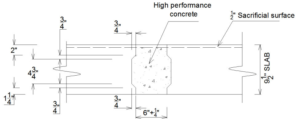
(a) Deck slab and connection dimensions
