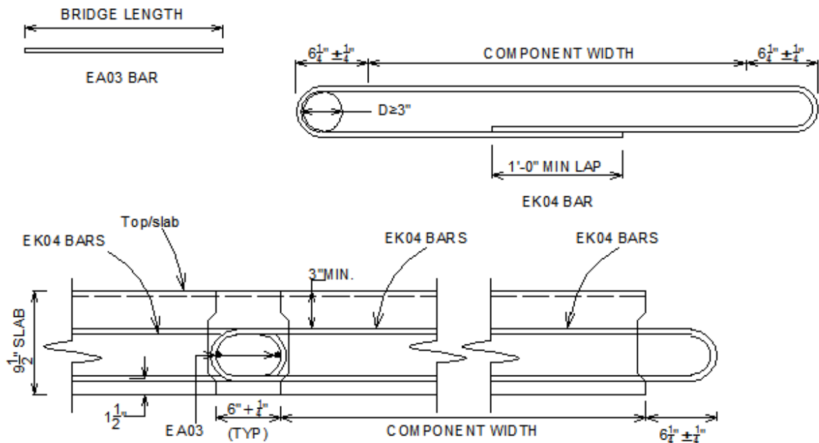
(a) Deck slab and connection dimensions
