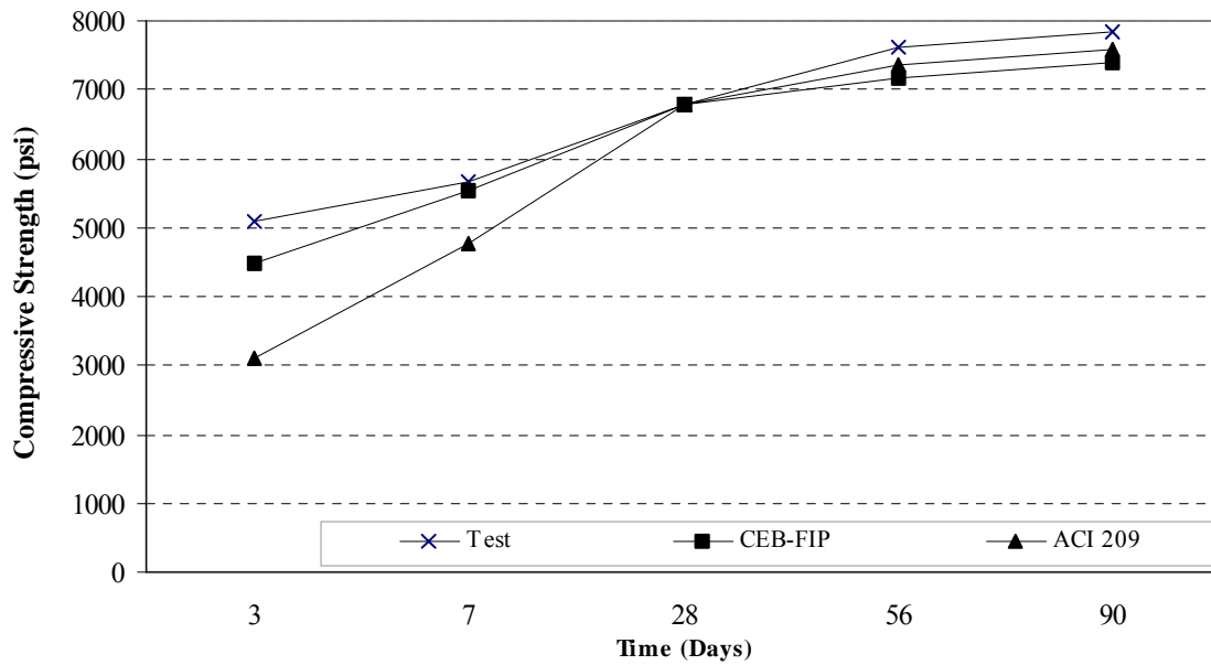
Figure 7-4. Compressive strength variation against time (S05 of 82025)
